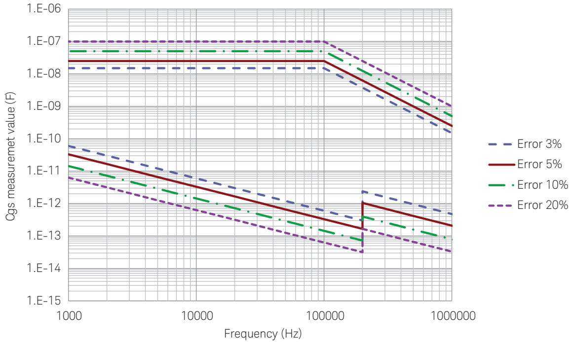
Cgs measurement accuracy 3-terminal Cgs:Cds:Cgd= 1:1:1
