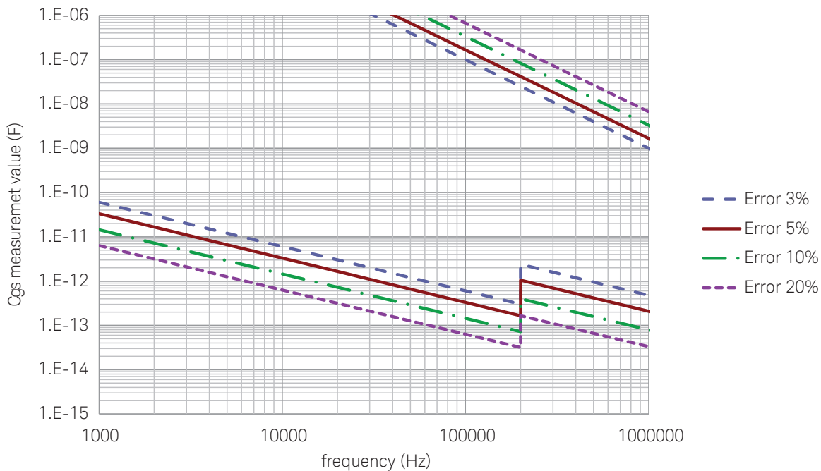
Cgs measurement accuracy 3-terminal Cgs:Cds:Cgd= 1:0.1:0.01
